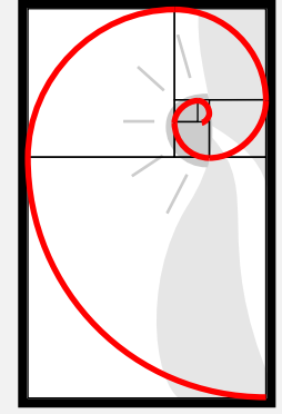
Fibonacci
